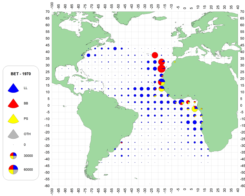
c. BET(1970-1979)
