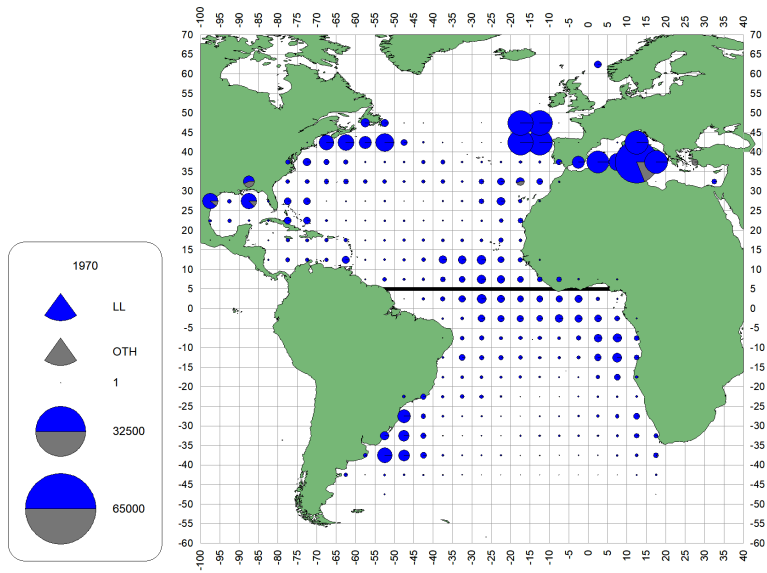
c. SWO (1970-79)
