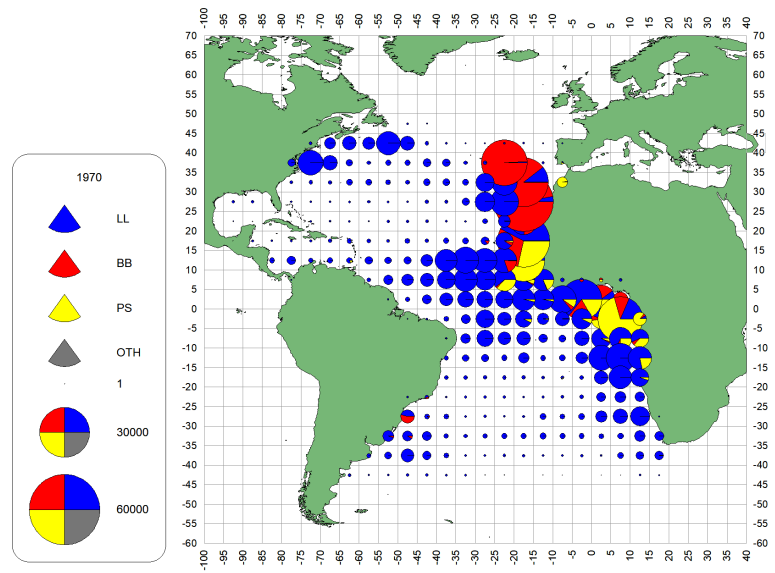
c. BET(1970-79)
