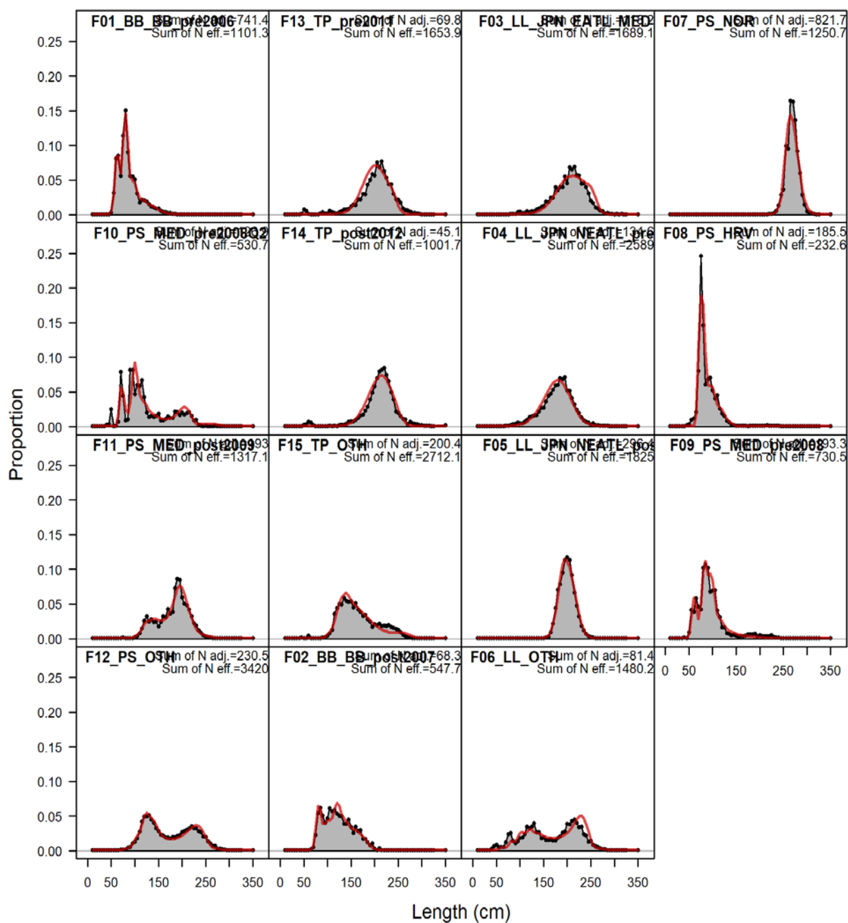
Figure 14. Stock Synthesis fits to East Atlantic bluefin tuna length compositions by fleet for the base run (run 16 reweight). The grey distributions show the observed aggregated length composition by fleet and the red line shows the model predicted length composition.
