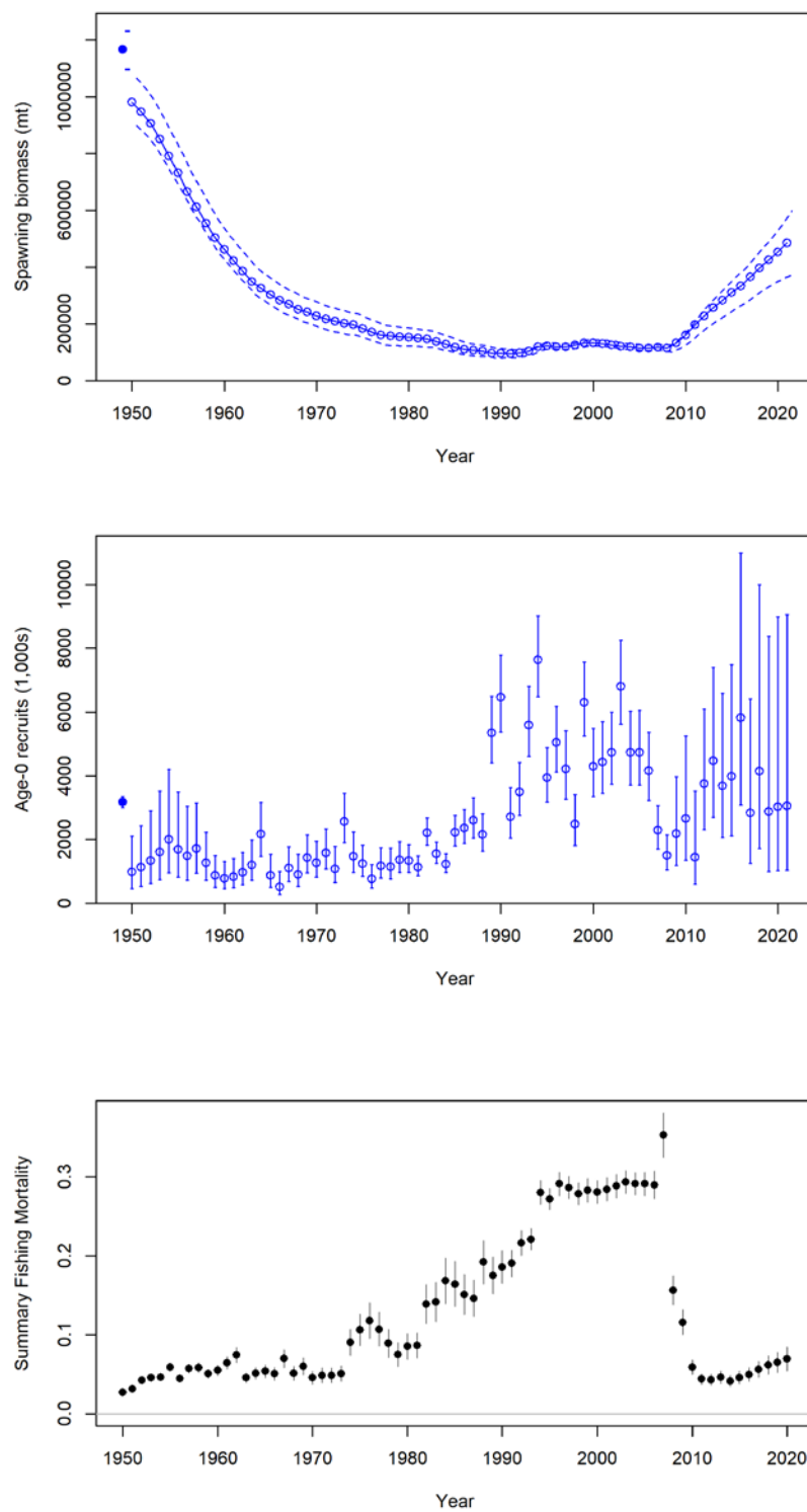
Figure 25. The time series of spawning stock biomass (SSB), fishing mortality (biomass exploitation rate was used as a proxy), and recruitment (age 0) for the Stock Synthesis Run 16 reweight.
