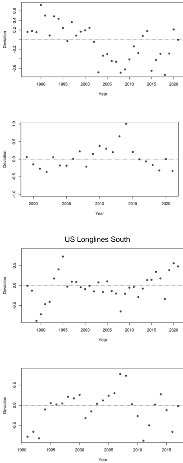
Figure 9. Stock Synthesis model fit residual errors around North Atlantic albacore indices of relative abundance.
