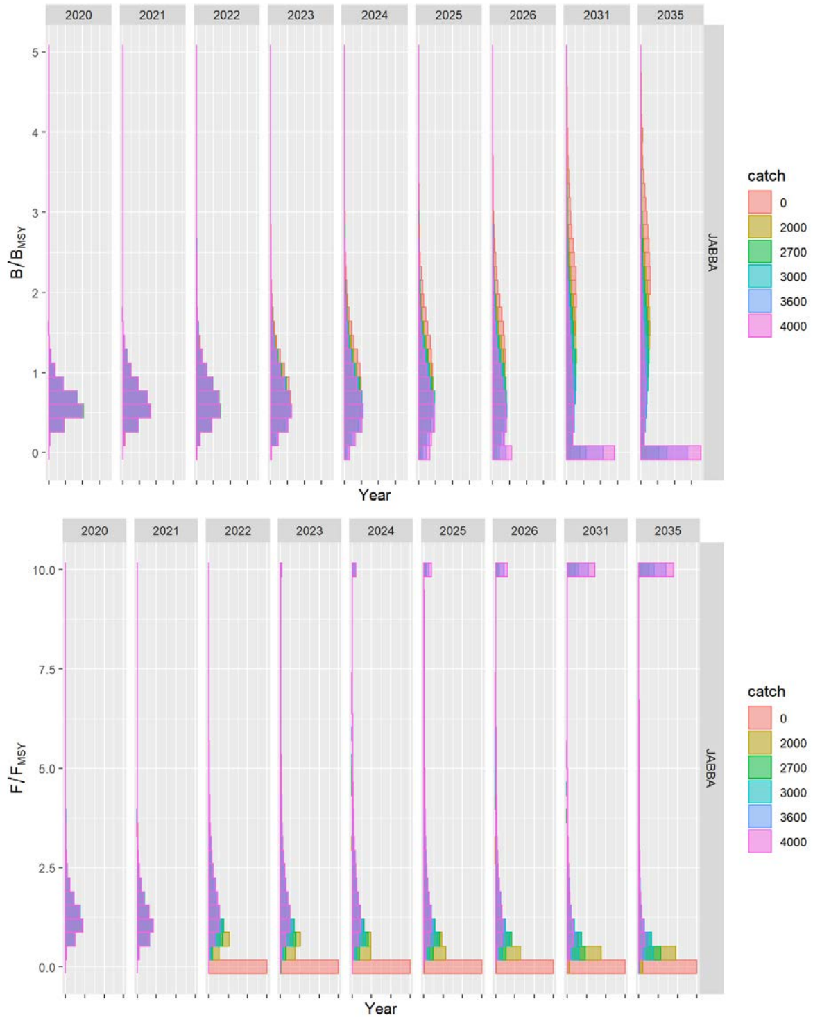
Figure 18. Posterior distribution of projected relative stock biomass (upper panel, B/B_{MSY} ) and fishing mortality (bottom panel, F/F_{MSY} ) of Mediterranean albacore for selected projection years of 2020-2035 and for selected fixed catch scenarios of 0 – 4,000 tons, based upon the projections of the JABBA final model (S4).
