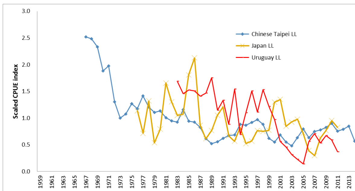
ALB-Figure 7. South Atlantic albacore. Standardized catch rates used in the 2016 stock assessment.
