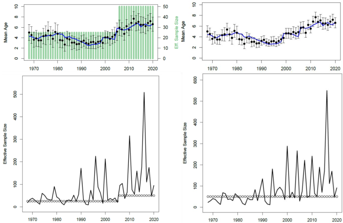
Figure 5. Assumed effective sample size for fishery age composition (green bars, top; open circles, bottom), observed mean age (closed circles and error bars, top) and model estimates of mean age (blue line, top) and effective sample size (black line, bottom) from the single-fleet ASAP application to Eastern Atlantic and Mediterranean Atlantic Bluefin tuna; unrevised data (left) and revised data (right).
