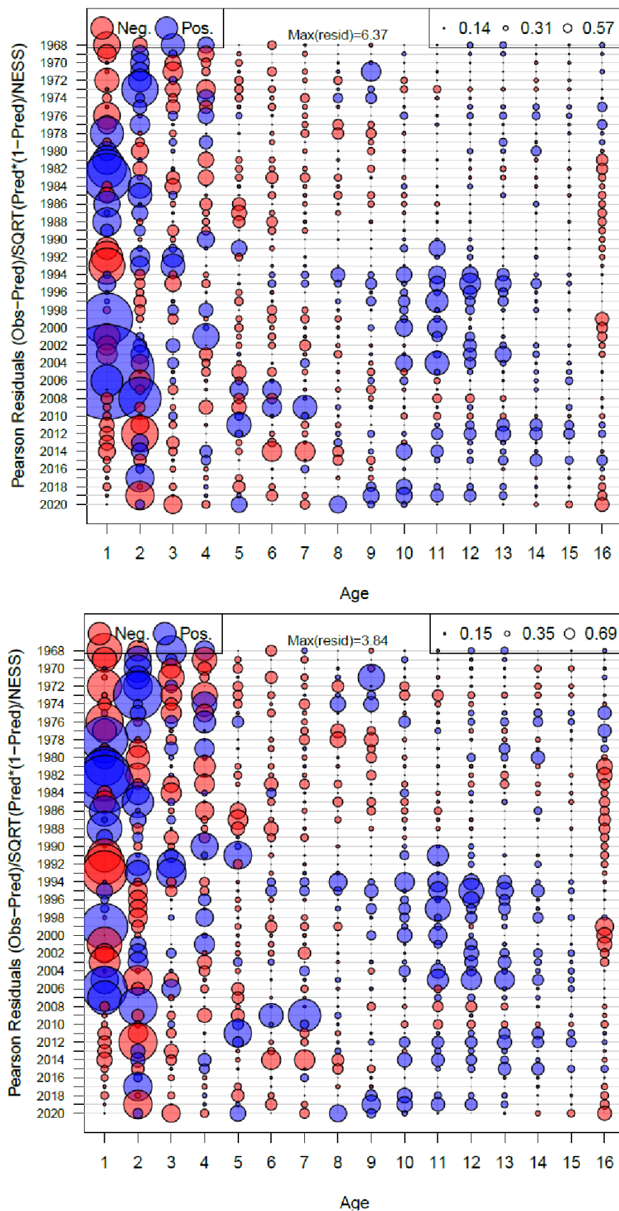
Figure 8. Pearson residuals of fishery age composition from single-fleet ASAP application to Eastern Atlantic and Mediterranean Atlantic Bluefin tuna, from unrevised data (base1, top) and revised data (base2, bottom).
