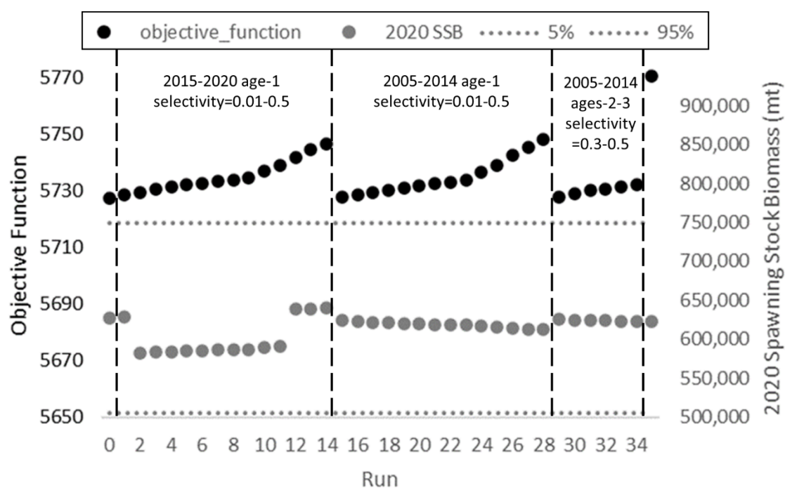
Figure 11. Sensitivity of objective function (black dots) to starting values for recent selectivity of young ages and terminal stock estimates (grey dots) with 90% confidence limits of base estimate (dotted horizontal lines). Run 0 is the single-fleet ASAP base2 run and run 35 is an alternative run with naïve starting values (0.5) for all selectivity estimates.
