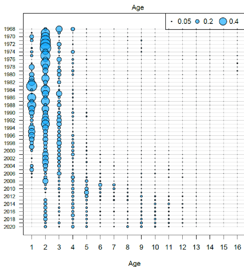
Figure 2. Age composition of Eastern Atlantic and Mediterranean Atlantic Bluefin tuna catch; unrevised data (top) and revised data (bottom).
