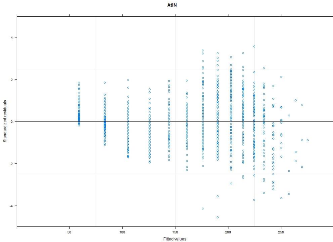
Figure 2. Residuals from different strata von Bertalanffy fits (strata definition in main text).
