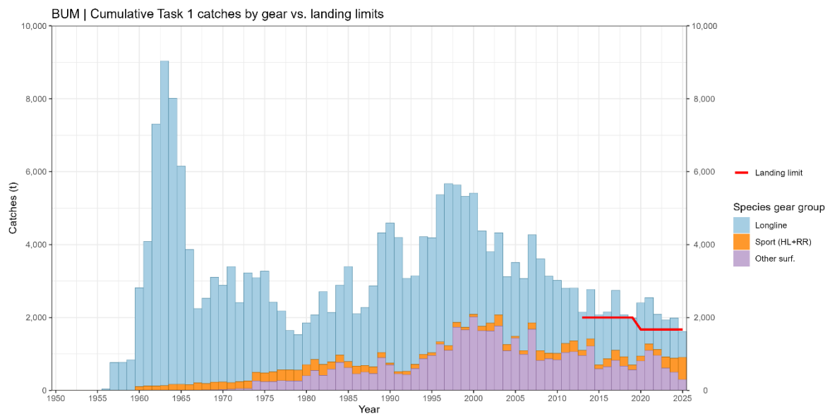
Figure 2. Blue marlin Atlantic (BUM-A stock) total reported and estimated catches (landings and dead discards, t) by year and major gear. Data as of 18 September 2026.
