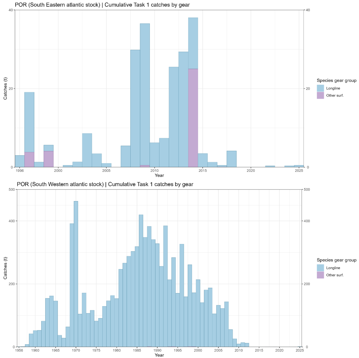
Figure 3. Porbeagle shark southeastern and southwestern Atlantic stocks (POR-SE and POR-SW, respectively in top and bottom figures) total reported and estimated catches (landings and dead discards, t) by year and major gear. Data as of 18 September 2026.
