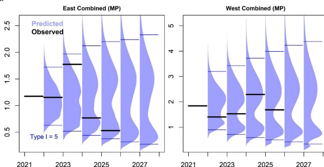
Figure 19.15.1 Standard marginal plots of observed composite indices (black bars) and distribution of posterior predicted data (blue density distribution) for the reference grid of OMs (n =2304, 48 OMs, 48 simulations each). Blue bars represent the 95% intervals. The Moroccan-Portuguese trap data points between 2023 and 2025 were not used due to changes in temporal distribution of the catches that created immediately unsolvable problems for the existing index standardization.
