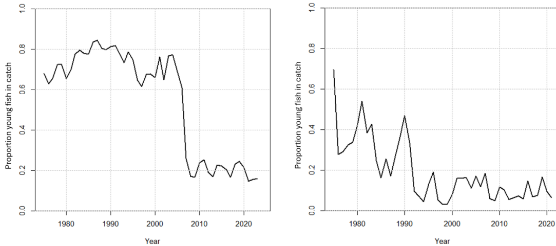
Figure 4. Estimated proportion (in numbers) of young fish (ages 0-3) in catches for the East Atlantic and Mediterranean bluefin tuna (left) and the West Atlantic (right) stocks.
