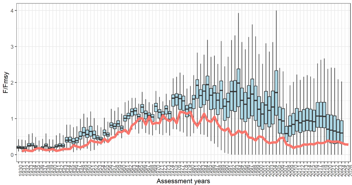
Figure 19.8.4 Relative fishing mortality ( F/F_{MSY} ) estimated in the MPs of the MSE (boxplot, boxes represent 50% CI and whiskers 95% CI) and estimates from the 2026 MP model (solid line).
