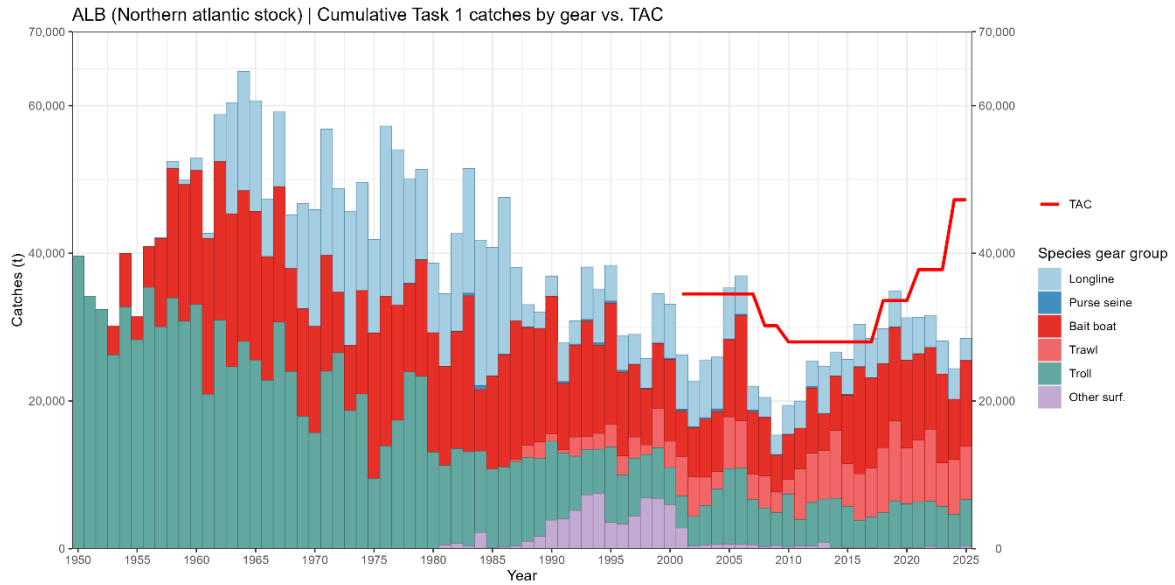
Figure 2. Albacore northern Atlantic stock total reported and estimated catches (landings and dead discards, t) by year and major gear. Data as of 18 September 2026.
