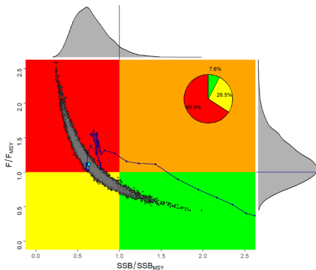
Figure 1. Kobe plot for the Mediterranean swordfish stock status trajectories in 2024, estimated during the 2026 stock assessment. The inserted pie chart indicates the probability of the stock being within each Kobe colour quadrant. The probability distributions shown in each axis represent uncertainty around current SSB/SSB_{MSY} and F/F_{MSY} . The black line indicates the stock status trajectory starting in 1982.
