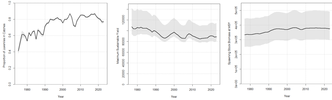
Figure 3. Estimated proportion (in numbers) of juveniles (ages 0, 1 and 2) in catches of bigeye tuna over time (left plot) compared to the time-dynamic estimates of MSY (center plot), and dynamics spawning stock biomass at MSY (right plot). Shade area represents the 80% confidence intervals of the uncertainty grid assessment model.
