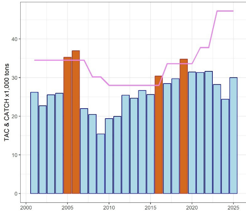
Figure 19.8.1 ALB-N reported catch (Task 1NC, bars) and TAC (solid line). Brown bars indicate years when the catch exceeded the TAC. Note that TAC established with the ALB-N harvest control rule or the MP started in 2018.
