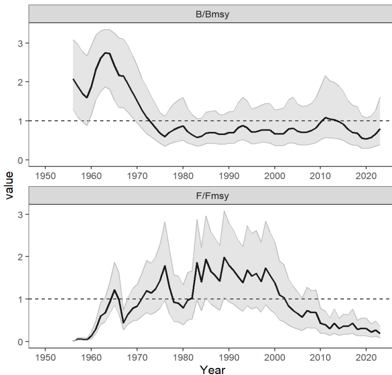
Figure 3. Trajectories of biomass relative to B_{MSY} ( B/B_{MSY} ) at the end of the years and fishing mortality relative to F_{MSY} ( F/F_{MSY} ) for the final base case model for the Atlantic white marlin, the shaded area indicates the 95% CRI bounds.
