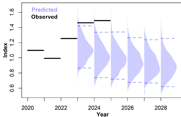
Figure 19.19.1 Observed values of the combined index (black lines) relative to simulated values projected from 2023 to 2028.
