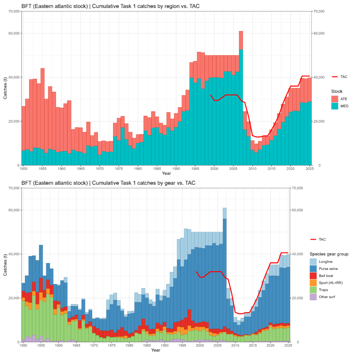
Figure 1. Reported catch for the East Atlantic and Mediterranean from Task 1 data from 1950 to 2025 split by main geographic areas (top panel) and by gears (bottom panel) together with unreported catch estimated by the Committee from 1998 to 2007 and TAC levels since 1998. Data as of 18 September 2026.
