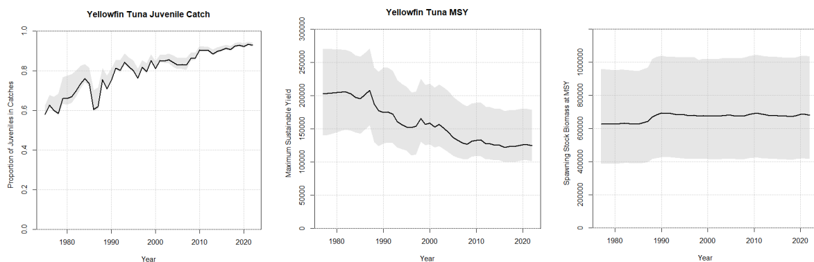
Figure 5. Estimated proportion (in numbers) of juveniles (ages 0, 1, and 2) in catches of yellowfin tuna over time (left plot) compared to the time-dynamic estimates of MSY (center plot), and dynamic spawning stock biomass at MSY (right plot). Shade area represents the 80% confidence intervals of the uncertainty grid assessment model.
