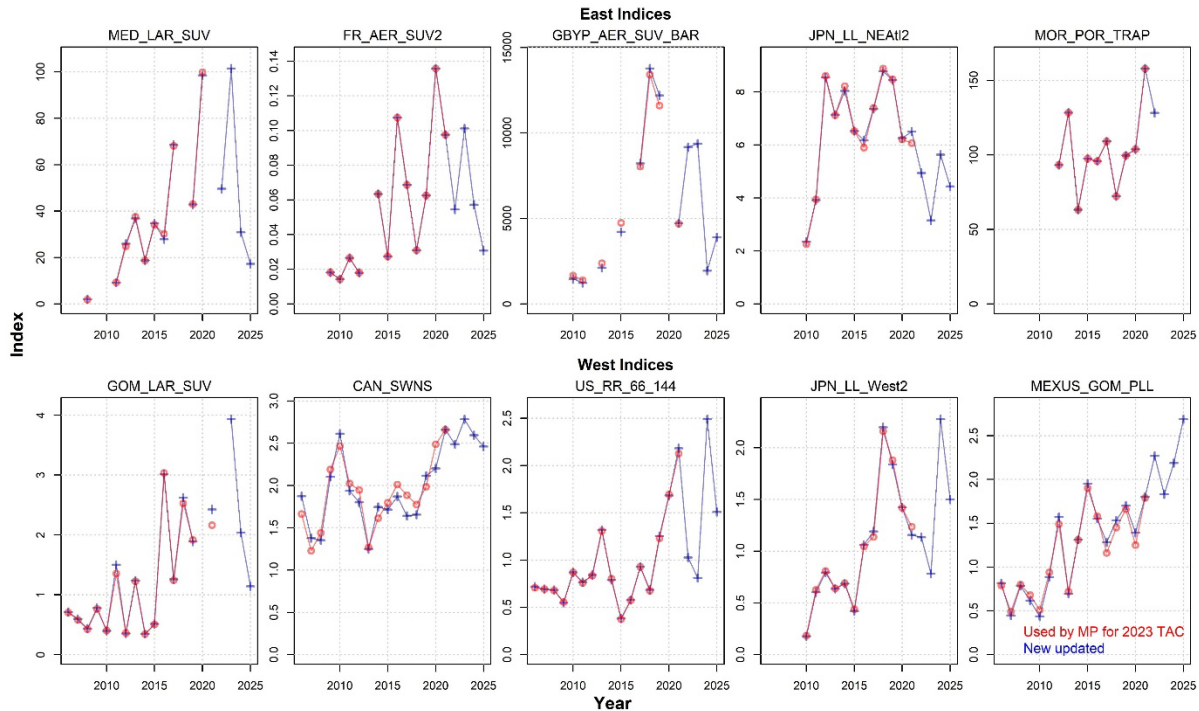
Figure 19.15.2 Plot of indices used in the 2022 MP calculation (red) and the new updated indices (blue) that were rescaled by the factor k and used in the MP calculations for 2026-2028 TACs. Red values are original indices used to determine the 2023-2025 TAC and in MSE conditioning; the blue values are strict updates of the indices through 2025. Within the past three years, the Moroccan-Portugal trap data points between 2023 and 2025 were not used.
