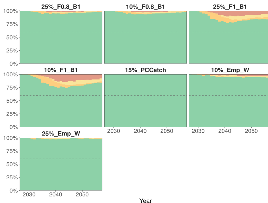
Figure 19.9.1. Time series of the estimated status of North Atlantic albacore under the seven CMPs evaluated in 2026 under the new MSE framework (reference set of operating models). For each year, colours indicate the probability of being in each of the Kobe quadrants. The dotted line indicates the 60% probability of being in the green quadrant of the Kobe Plot.
