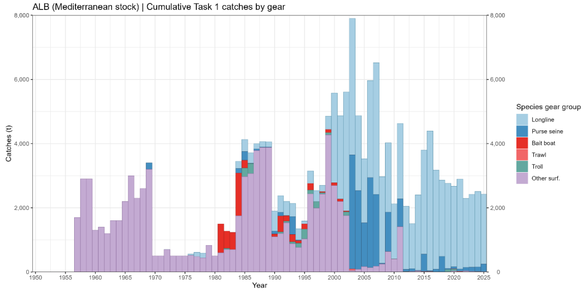
Figure 2. Albacore Mediterranean (ALB-M stock) total reported and estimated catches (landings and dead discards, t) by year and major gear. Data as of 18 September 2026.
