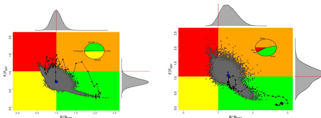
Figure 1. Kobe plot for the North (left) and South (right) Atlantic blue shark stock status in 2021, estimated during the stock assessment (Anon., 2023b). The lines indicate the stock status trajectory starting in 1971. The inserted pie charts indicate the probabilities of the stock being within each Kobe colour quadrant.
