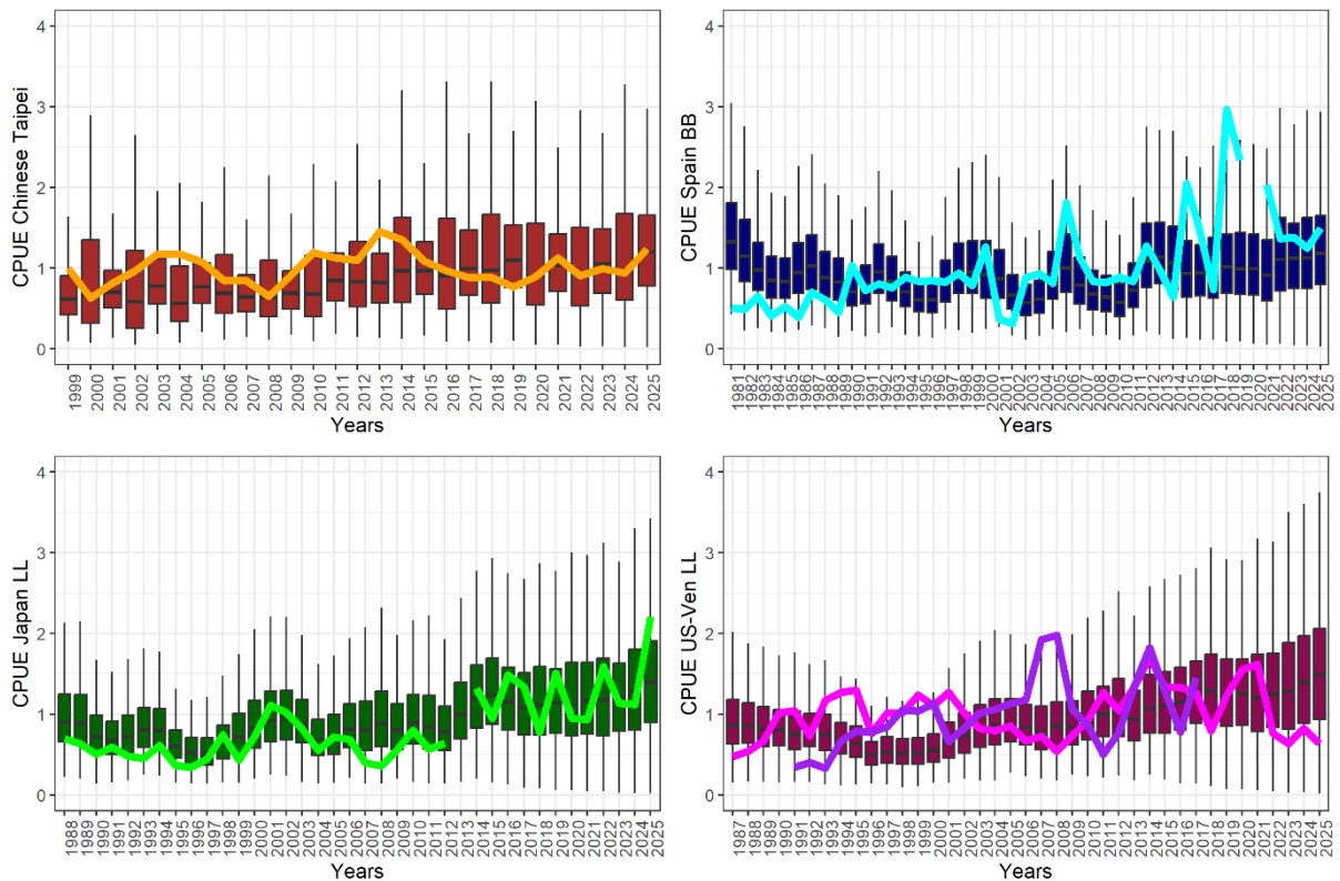
Figure 19.8.2 CPUE trajectories simulated in the MSE (boxplots) and standardized CPUEs (solid line) available in 2026.
