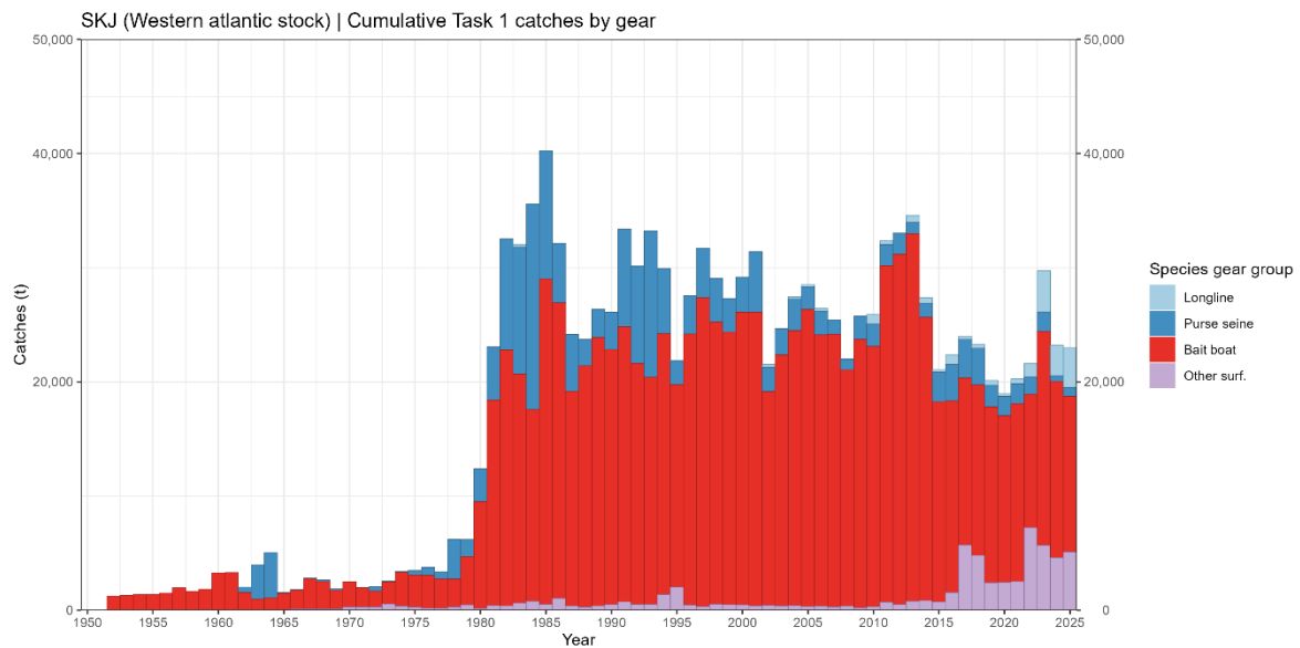
Figure 3. Skipjack West Atlantic (SKJ-W stock) total reported and estimated catches (landings and dead discards, t) by year and major gear. Data as of 18 September 2026.
