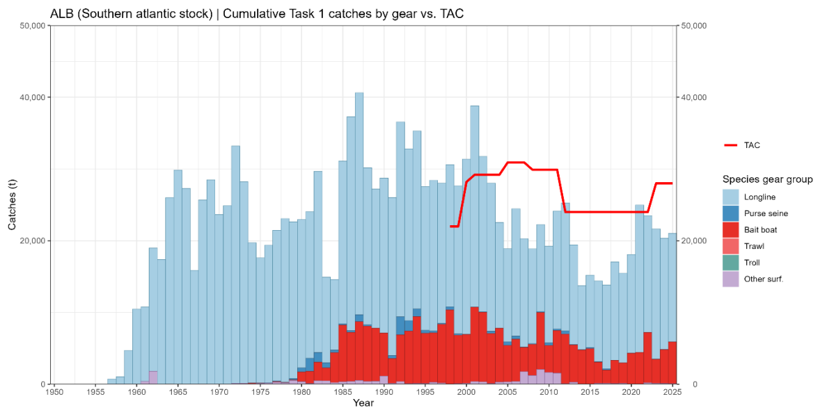
Figure 3. Albacore southern Atlantic stock total reported and estimated catches (landings and dead discards, t) by year and major gear. Data as of 18 September 2026.
