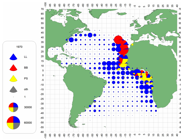
c. BET(1970-79)
