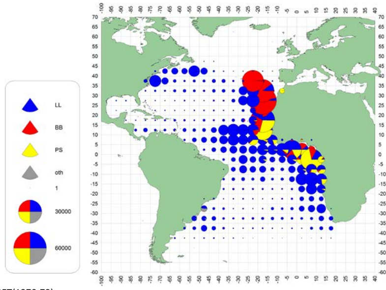
c. BET(1970-79)
