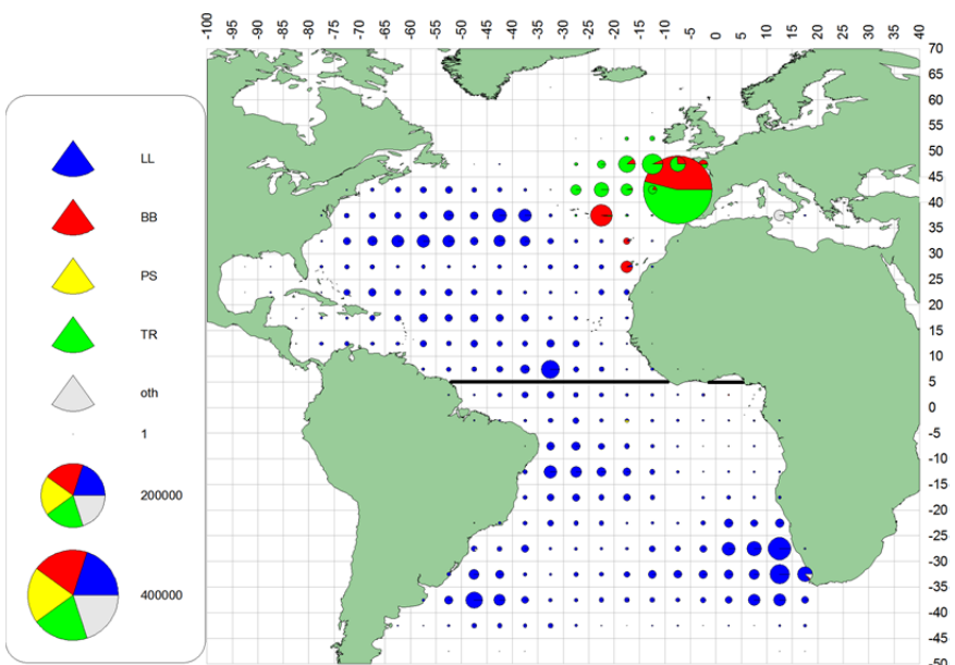
c. ALB(1970-79)
