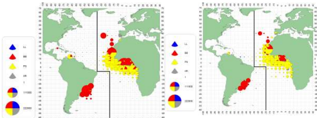
e. SKJ (2000-09)
