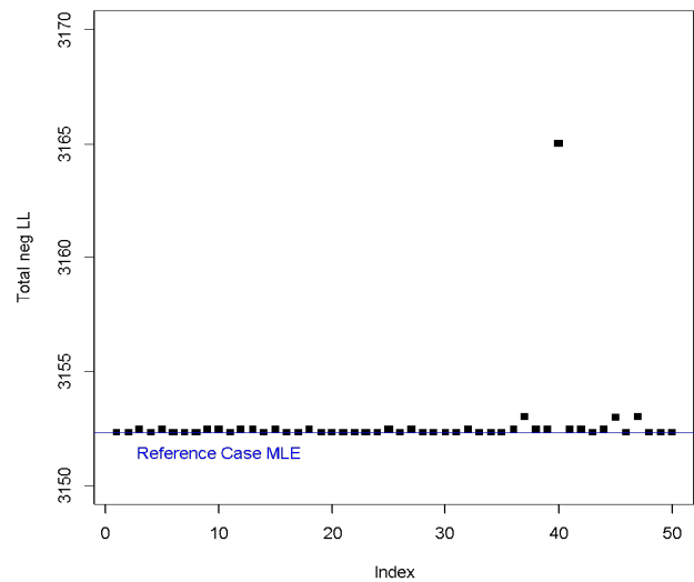
Figure 8. Final objective function (Total negative loglikelihood units) for the Stock Synthesis reference case across jittered starting parameter values.
