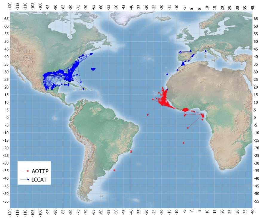
Figure 5 (C). Straight displacement from the release to the recovery position of the recaptured specimens in ICCAT conventional tagging on small tunas (including ICCAT AOTTP).
