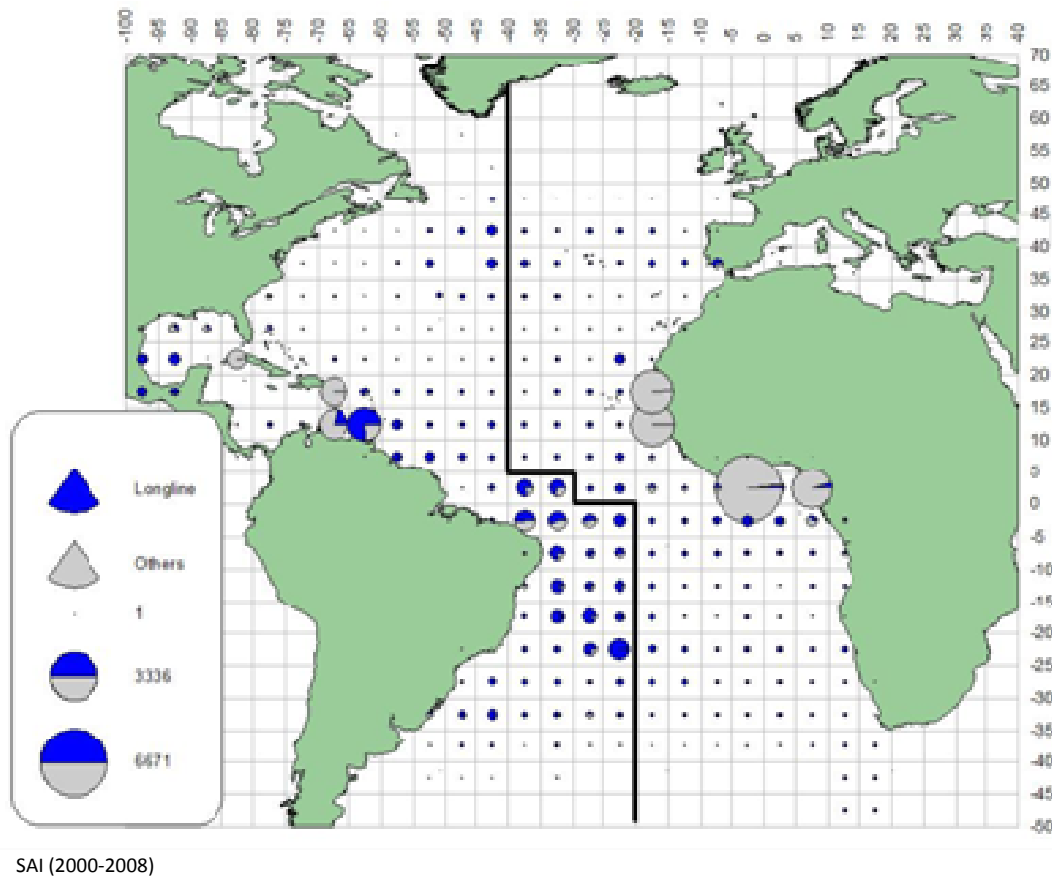
SAI-Figure 1. Geographic distribution of the mean sailfish catch (2000-2008) by major gears.
