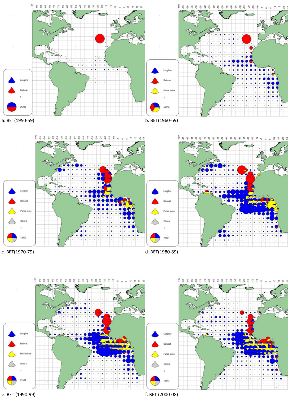
BET-Figure 1 [a-f]. Geographical distribution of BET catch by major gears and decade.
