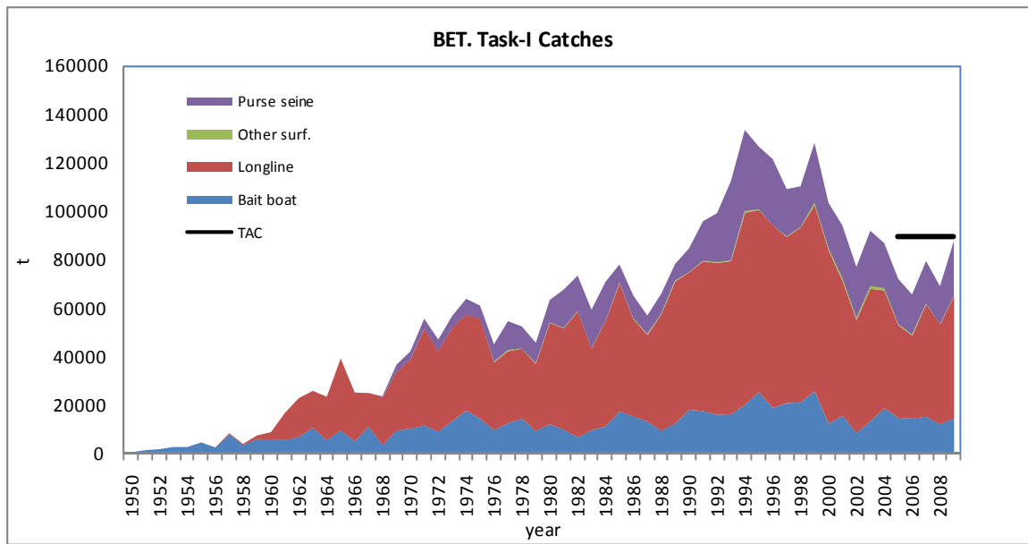
BET-Figure 2. Bigeye Task-I catches for all the Atlantic stock, in tons. Value for 2009 include estimates for a few fleets that had not yet reported data to ICCAT.
