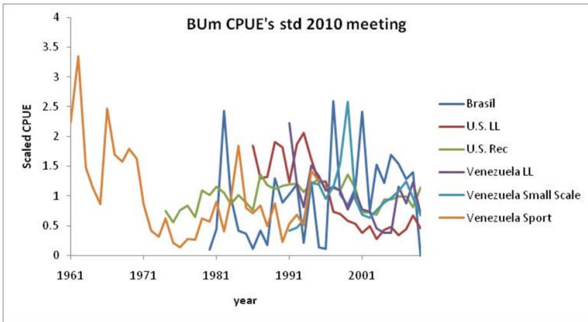
BUM-WHM-Figure 3. Blue marlin standardized CPUE's presented during the BUM data preparatory meeting. Some of the major offshore longline fleets are not included (i.e., Japan, Korea, and Chinese-Taipei).
