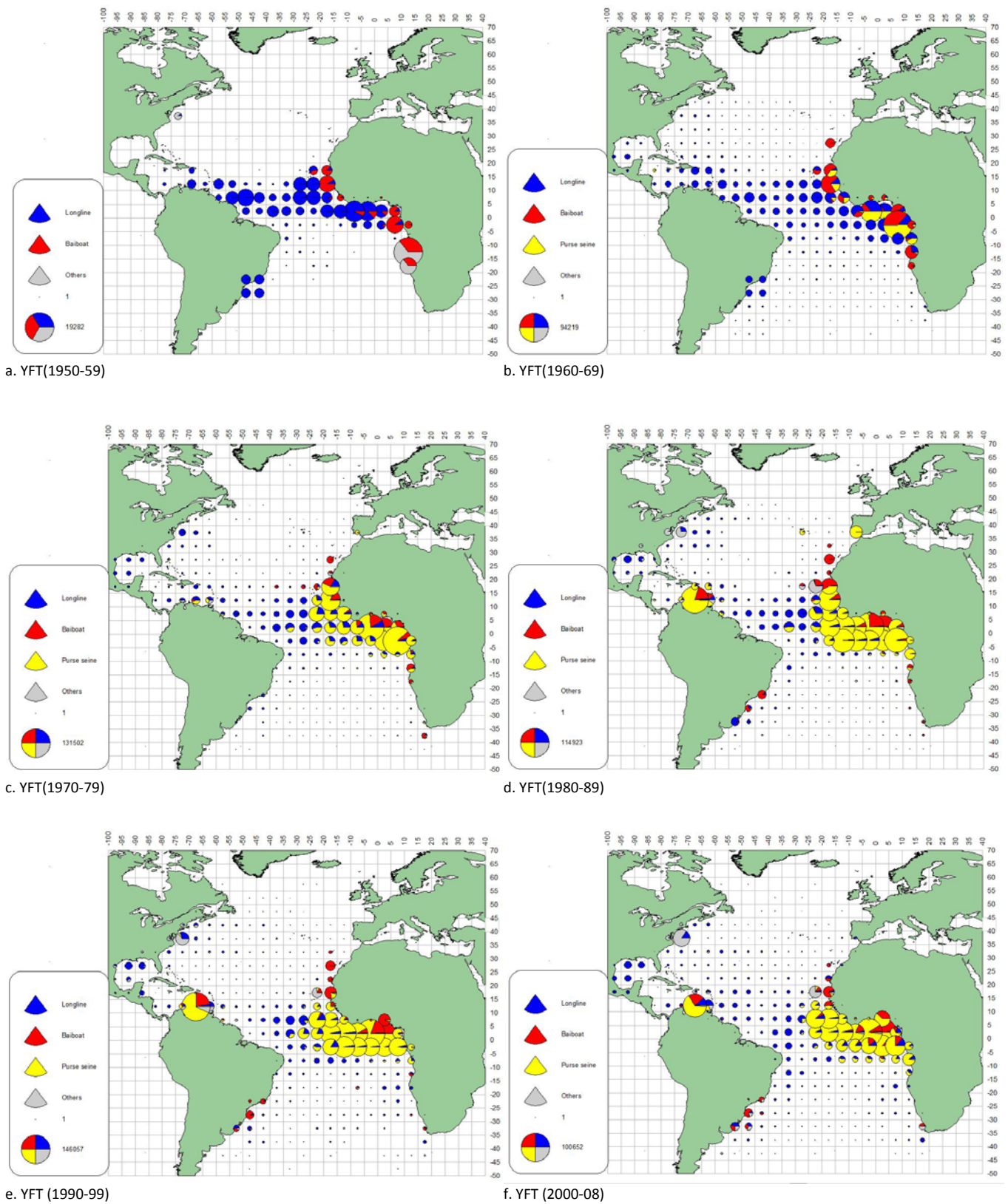
YFT-Figure 1 [a-f]. Geographical distribution of YFT catch by major gears and decade.
