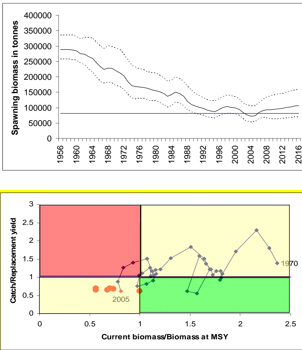
ALB-Figure 9. The upper plate indicates southern albacore spawning biomass over time, projections with a constant catch of 25,000 t over the next years and the reference SSB_{MSY} level with 80% confidence bounds. The lower plate indicates catch relative to replacement yield vs. current biomass relative to the biomass at MSY for the period 1970-2005. The circles are the current state of the stock for all the sensitivity runs.
