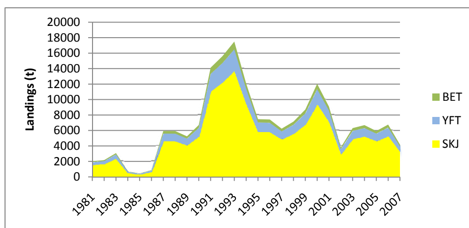
SKJ-Figure 5. Cumulative estimated landings of " faux poissons " for the three main species of tropical tunas in the local market of Abidjan (Côte d'Ivoire).
