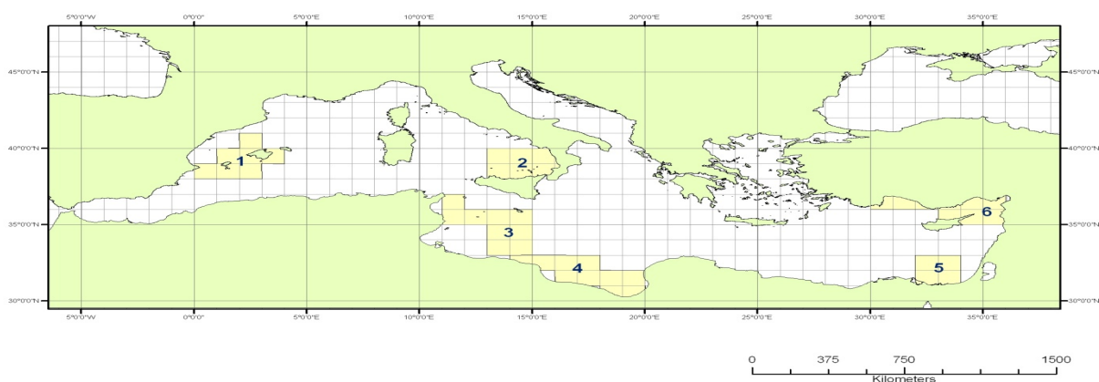
Figure 16.3. Spawning areas identified through analysis of VMS data used in the 2010 GBYP aerial survey program for surveying spawning biomass in the Mediterranean.
