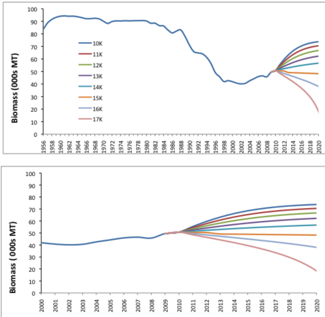
SWO-ATL-Figure 14. South Atlantic, projected biomass levels under various catch scenarios. The bottom panel provides the details of the projections over a reduced time interval.
