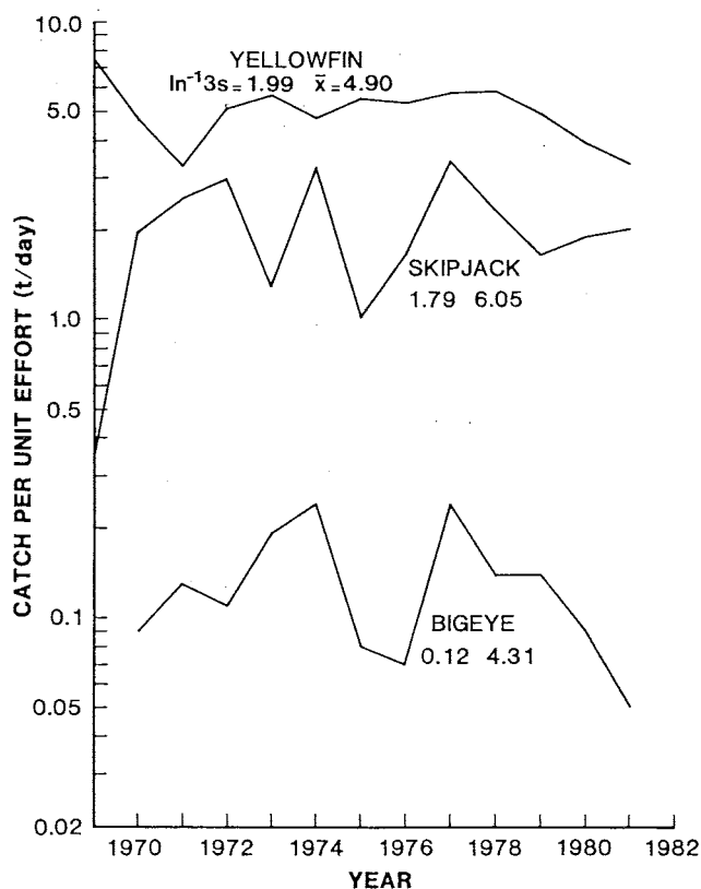
Figure 1. Catch per unit effort on logarithmic scale vs. year for skipjack, yellowfin, and bigeye tunas from the E. Atlantic large purse seiner fleet (Fonteneau et Cayré 1983). Geometric means ( \bar{x} ) and the measure of relative variability ( \ln^{-1} 3s ) are shown for each species.
