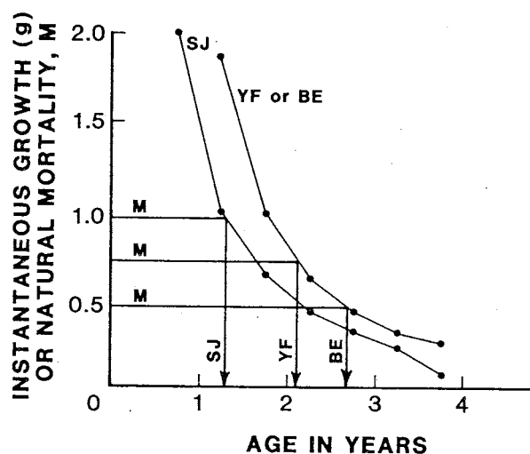
Figure 3. Instantaneous growth rate, g , vs. age as calculated for skipjack, yellowfin, and bigeye. Critical age is indicated by arrows, defining condition where g = \text{natural mortality} , M . Growth equations are by Joseph and Calkins (1969) and Hennemuth (1959b) for skipjack, Chatwin (1959) and Le Guen and Sakagawa (1973) for yellowfin, and Kume and Joseph (1966) and Morita (1973) for bigeye.
