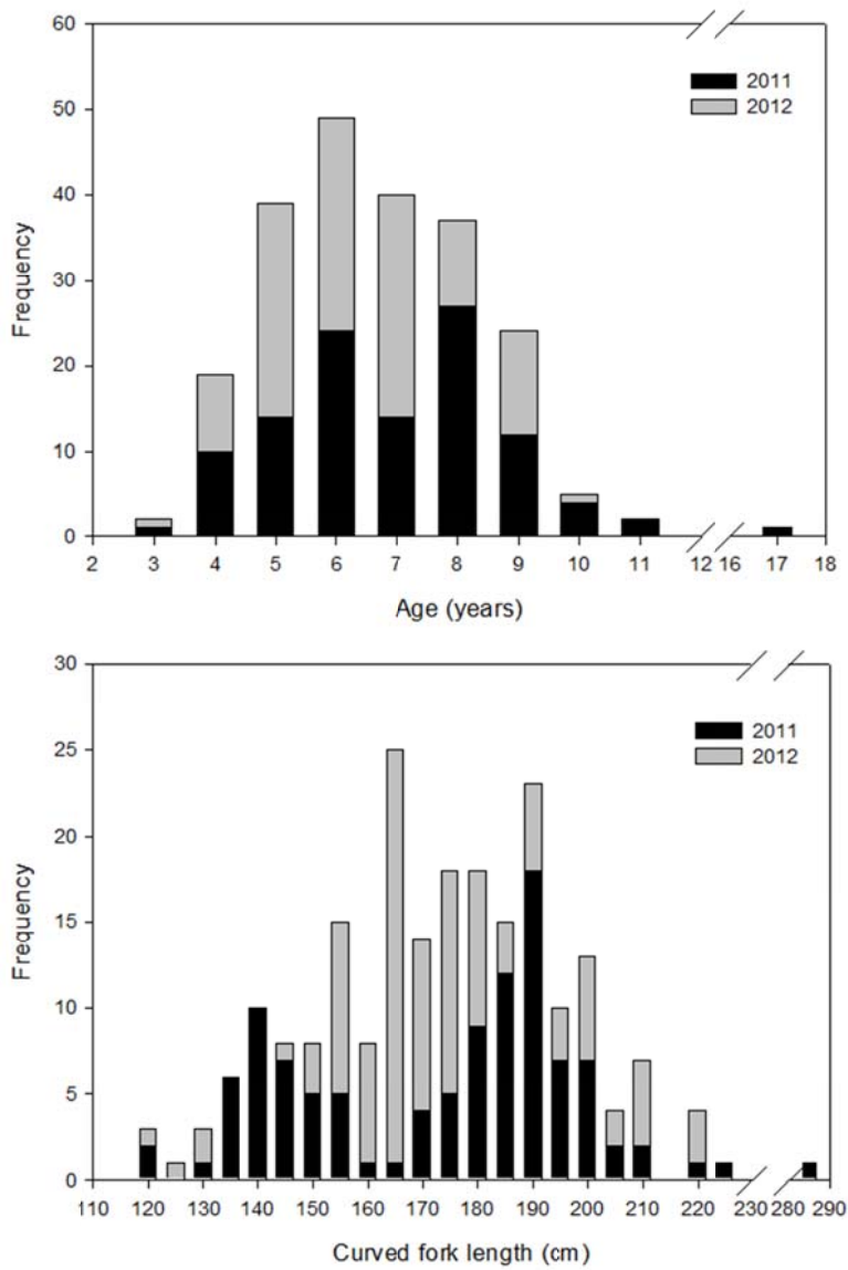
Figure 1. Age (top panel) and curved fork lengths (bottom panel) for North Carolina and Virginia Beach (US) Atlantic bluefin tuna sampled during January-April 2011 and 2012. Ages were estimated through enumeration of otoliths. Ages are presented by sampling year. The 2003 year-class is shown as age 8 and age 9 fish respectively for 2011 and 2012 samples.
