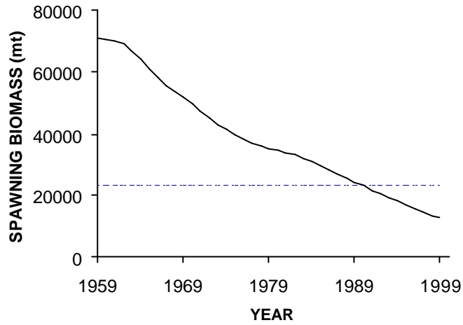
Figure 8. Estimated (modal) trends in spawning biomass from the fleet-specific model. Dashed horizontal line refers to the spawning biomass at MSY.
