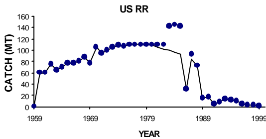
Figure 5. Model fits to fleet-specific catches.
