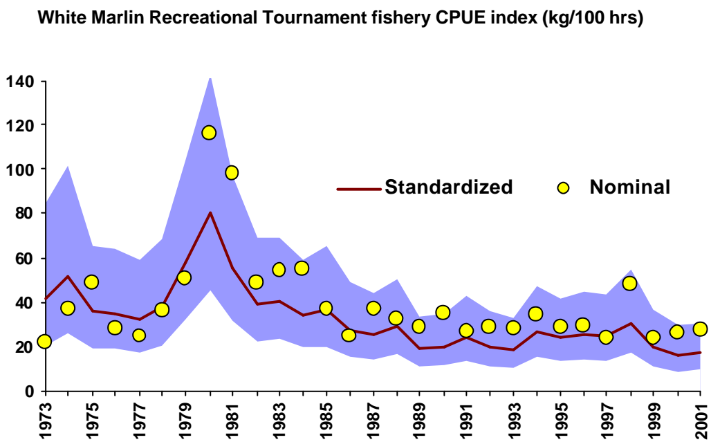
Figure 6. Nominal and standardized catch rates (CPUE) of white marlin from US recreational billfish marlin tournaments. Standardized series shows estimated upper and lower 95% confidence intervals, the solid line represents the overall average for the standard catch rate series.
