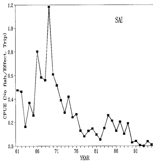
Fig. 1. Yearly standardized CPUE (No. Fish/effective effort) for billfishes at Playa Grande Yachting Club, Venezuela.
