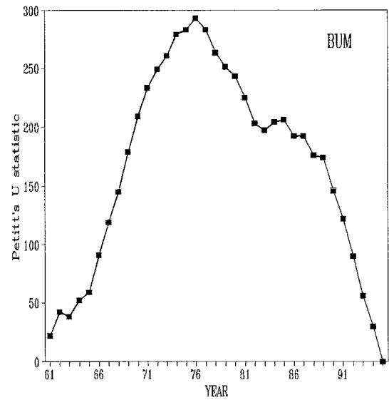
Fig. 2. Changes in the yearly Pettitt's statistics for billfishes at Playa Grande Yachting Club.
